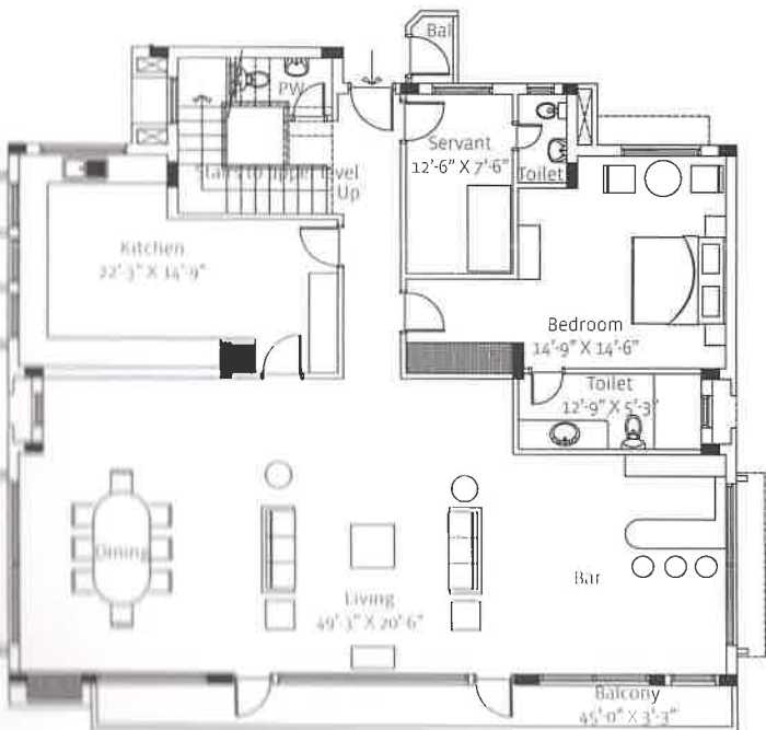
LOWER LEVEL
